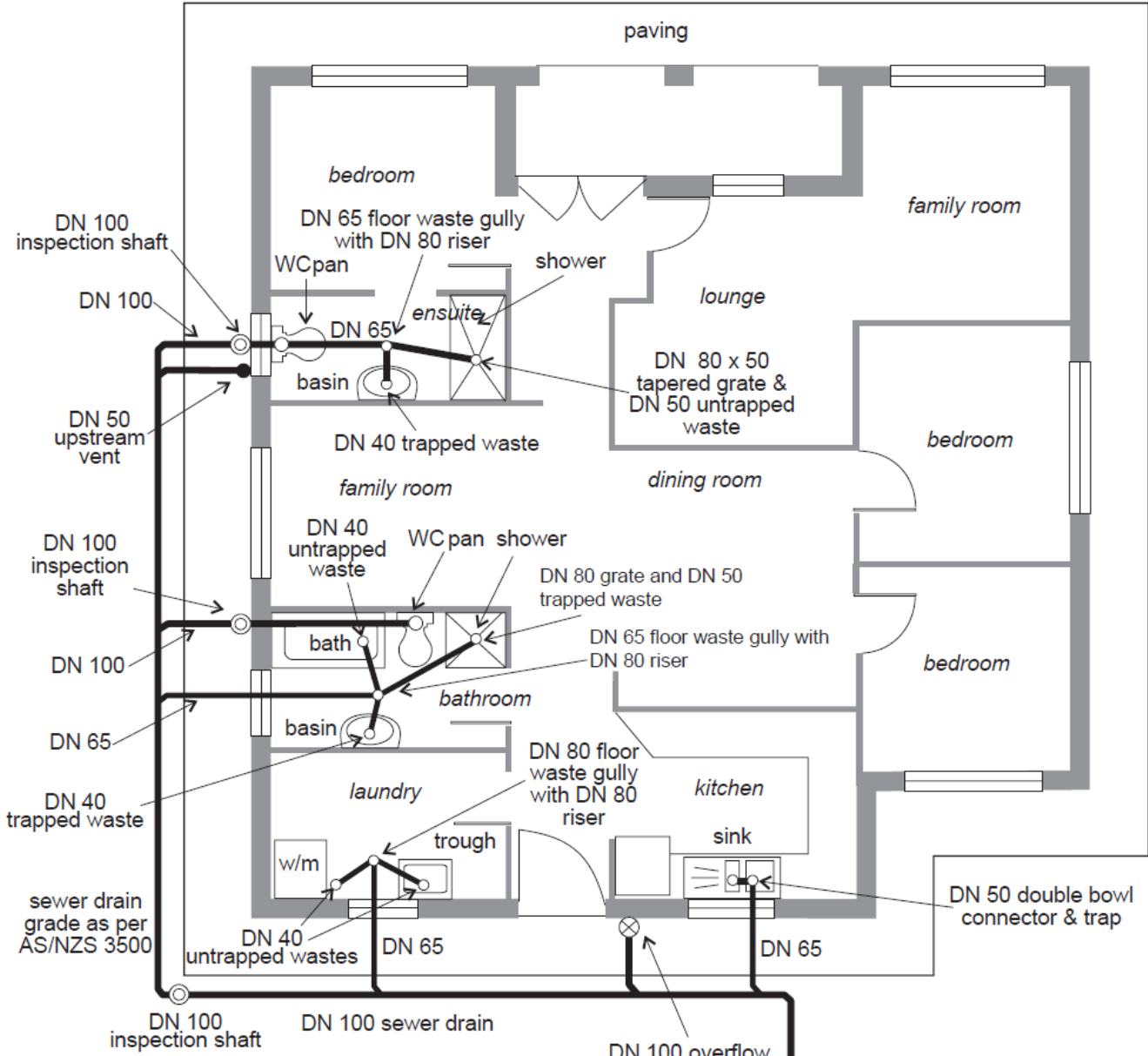
Figure 1: Typical building layout plan
